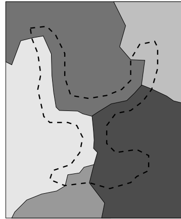
(b) Area redistributed amongst adjacent polygons
