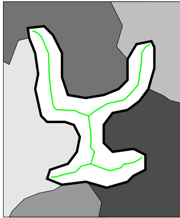
(a) Polygon (plus skeleton) selected for elimination
