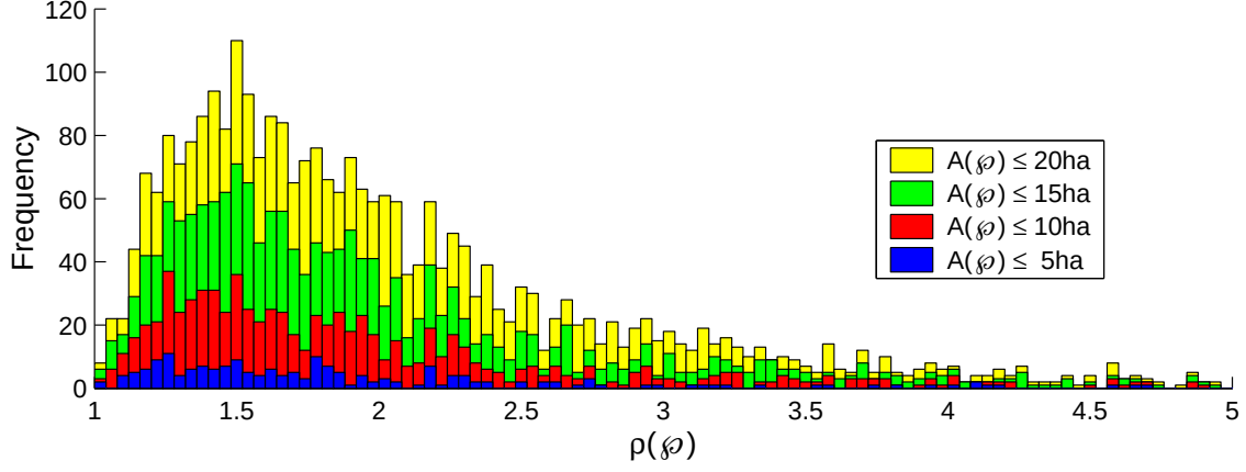
Figure 6: Histogram of \rho(\phi) for North Island NZLRI Polygons
